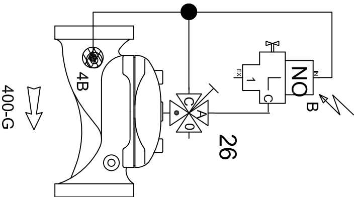
End gun valve with three way tap and BERMAD solenoid
